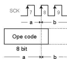
Figure 50. WREN/WRDI cancel valid timing
