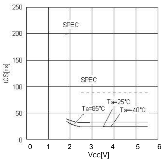
Figure 18. \overline{\text{CS}} high time tCS
