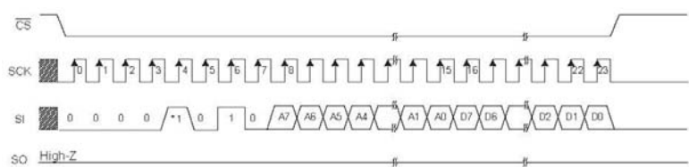
Figure 37. Write command (BR25L010/020/040-W)
